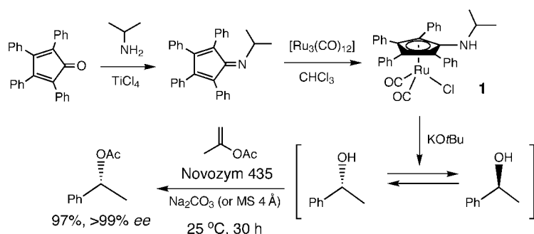
Scheme 1. Synthesis of 1 and DKR of 1-phenylethanol; MS = molecular sieve.
